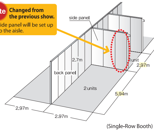
(Single-Row Booth)
